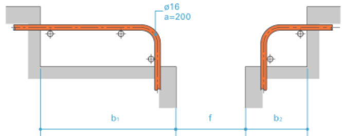
Figure 11 – Support system
